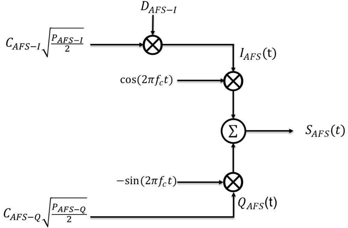
Figure 2: Modulation Scheme for AFS Signal
