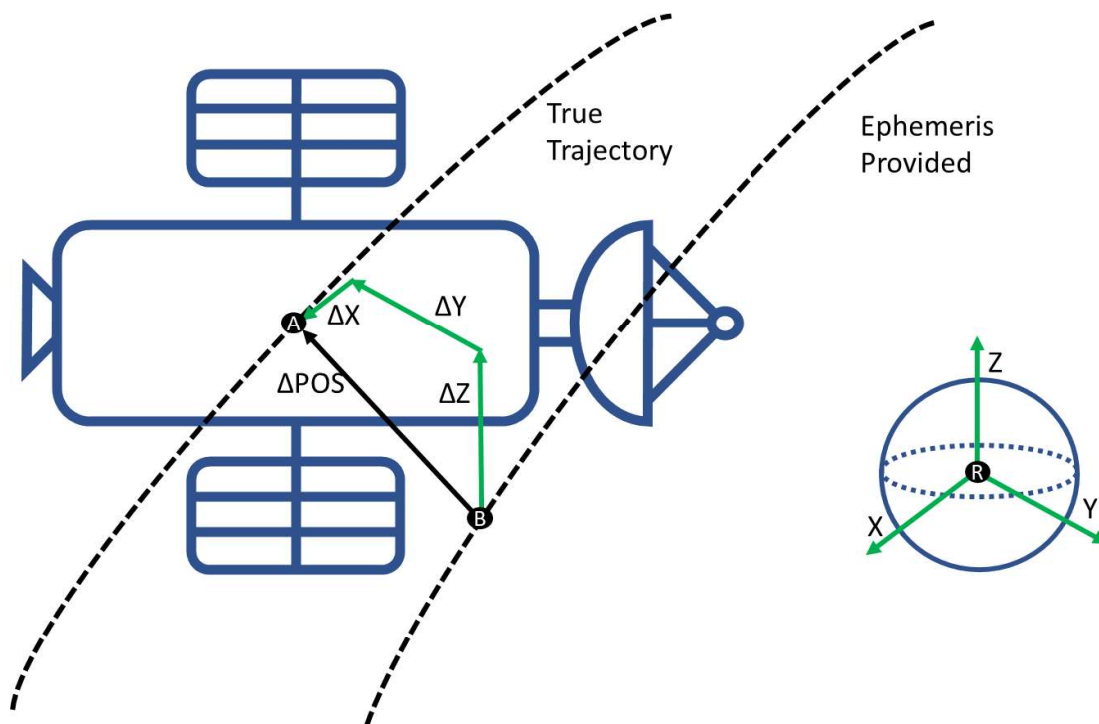
Figure B- 1: Representative illustration of ephemeris errors
