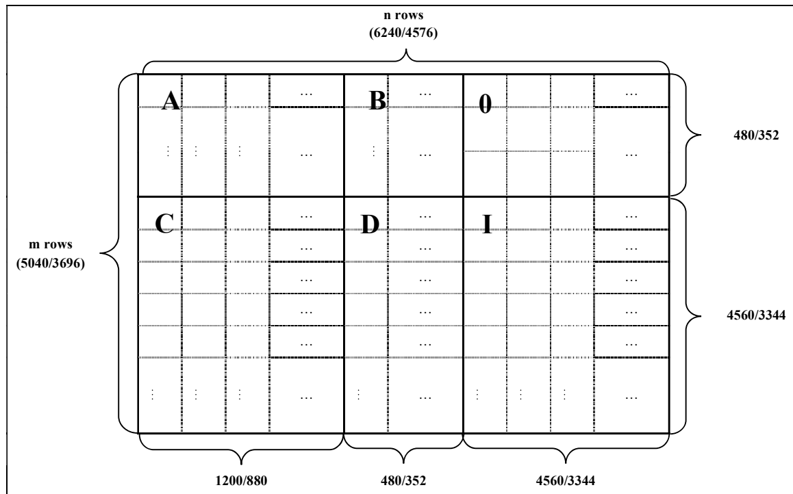
Figure 10: LDPC Submatrices
